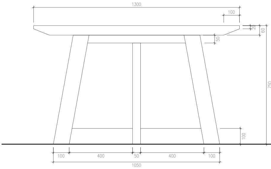
ROUND DINING TABLE - SIDE/FRONT VIEW SCALE 1:10
