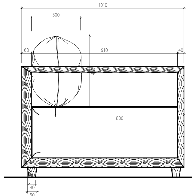
SINGLE SEATER - SIDE VIEW SCALE 1:10
