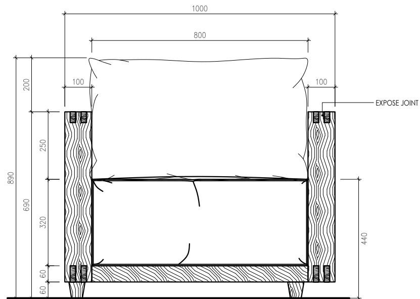
SINGLE SEATER - FRONT VIEW SCALE 1:10
