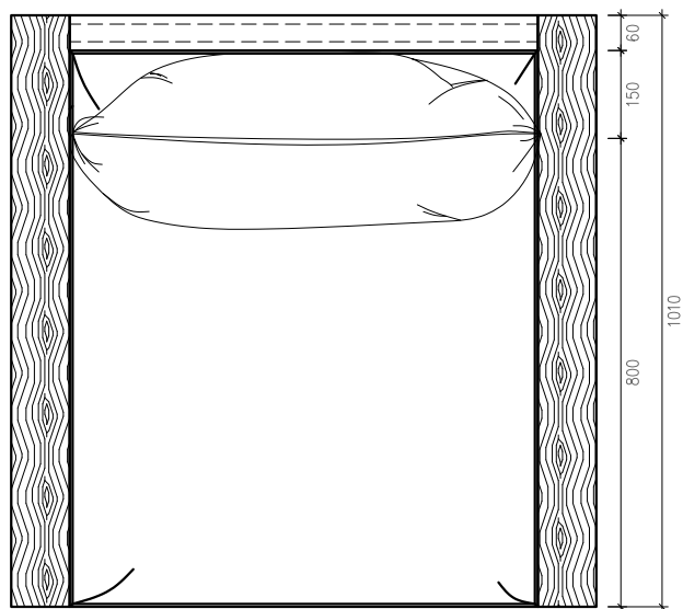
SINGLE SEATER - TOP VIEW SCALE 1:10
