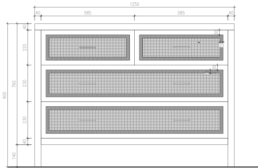
CREDENZA - FRONT VIEW SCALE 1:10
