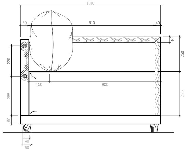
3-SEATER SOFA - SIDE VIEW SCALE 1:10
